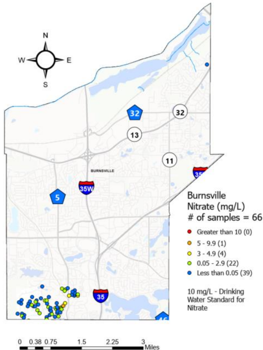
Figure 2. Nitrate results in untreated water from outside spigot
