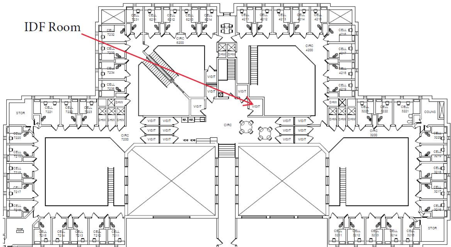
Figure 2 - Partial Floor Plan for Upper Level of Law Enforcement Center
