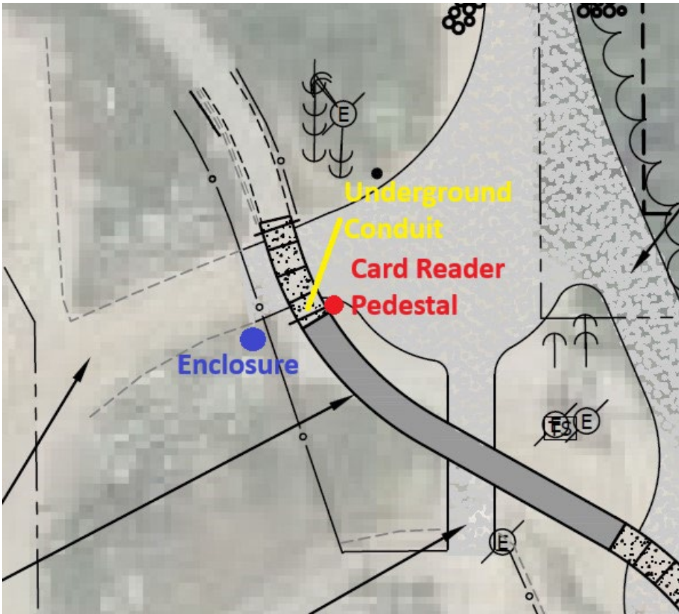
Figure 1 - Enclosure, Conduit, and Pedestal Locations
