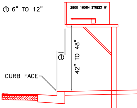
Location of Mailbox Post
